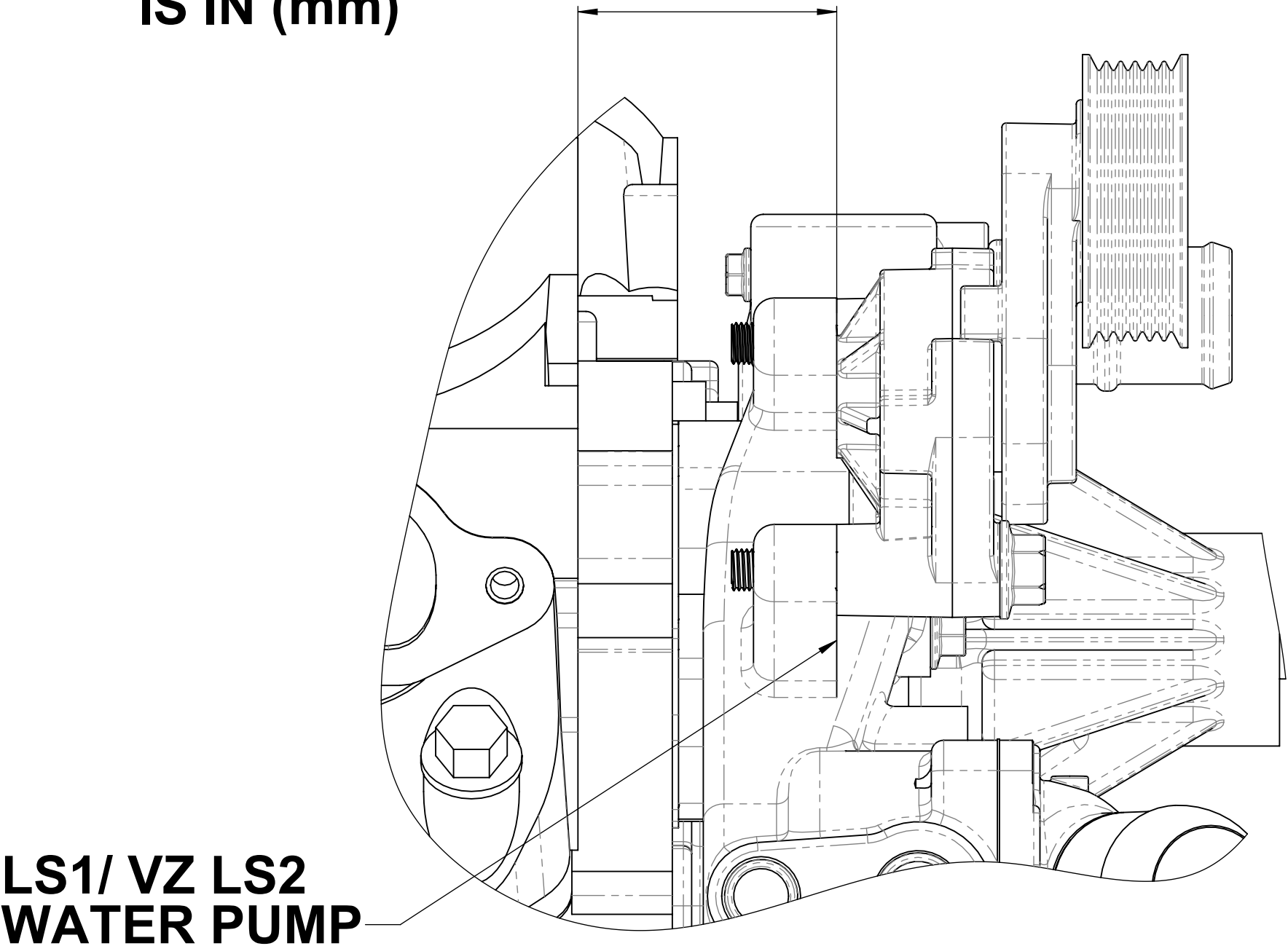
SIDE VIEW (2)
